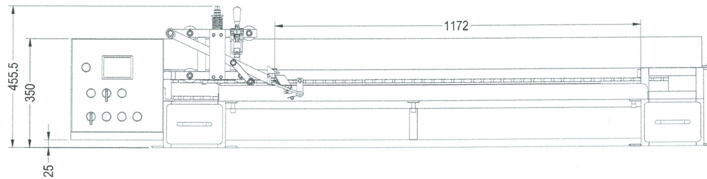
Front view
