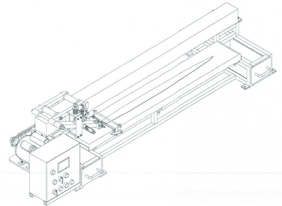
Isometric view
