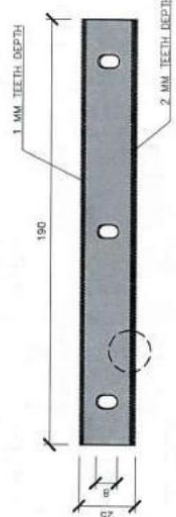
4 A-4 BLADE DETAILS
