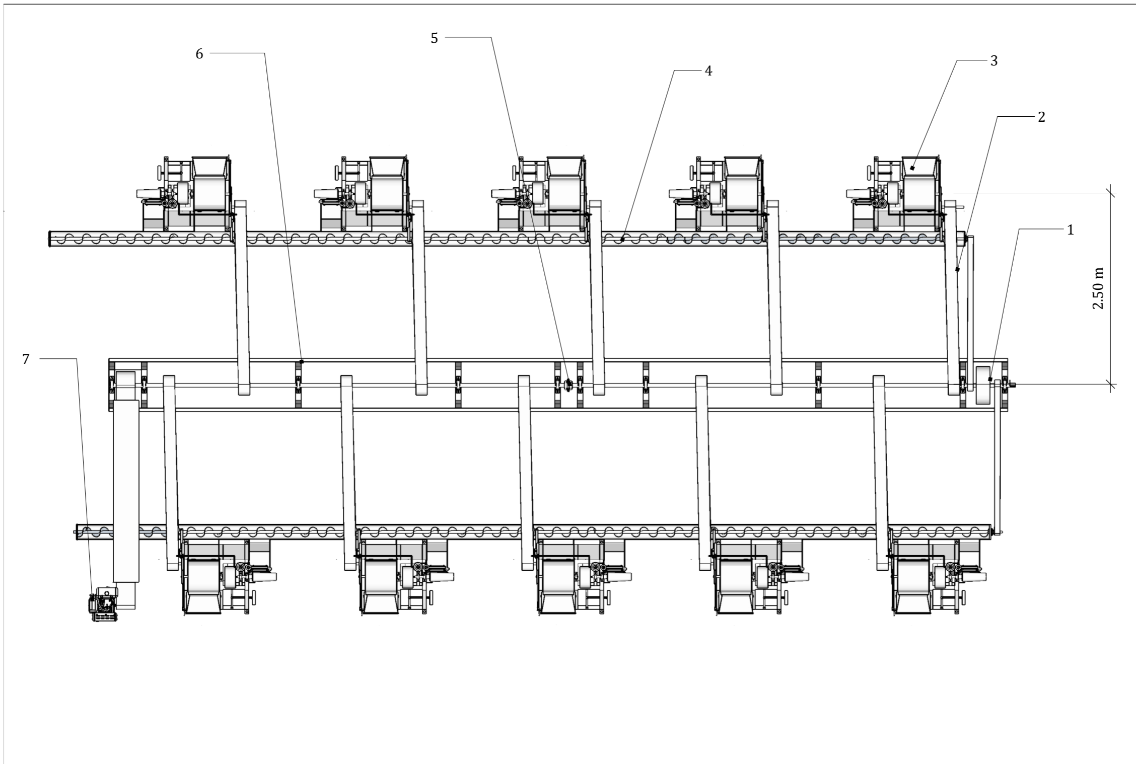
TOP VIEW Scale 1:50 mm
