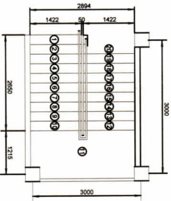
2 PLAN OF STAIR A-3 SCALE 1 : 60 M.
