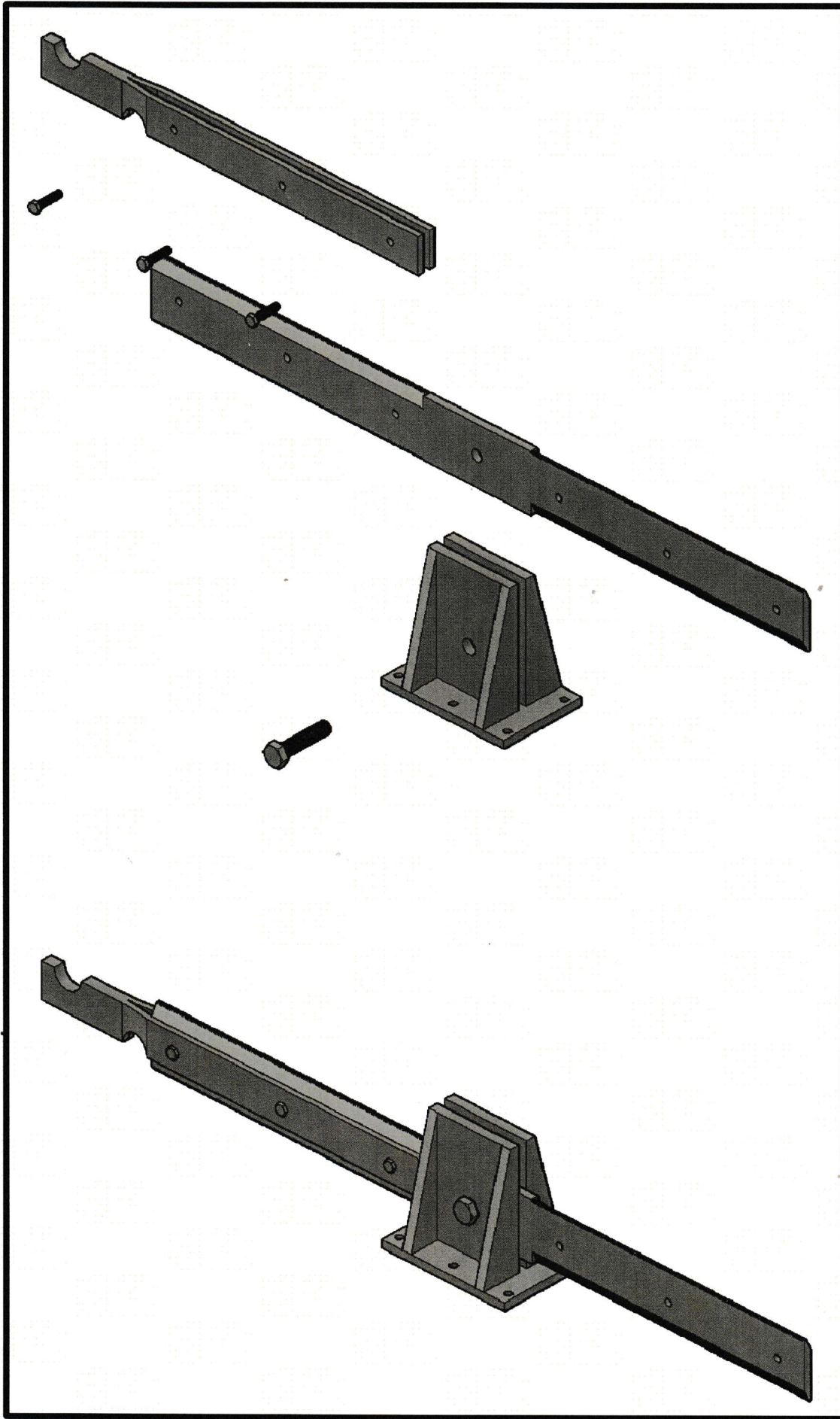
MASK Isometric view SCALE(20/30) SCALE(A3)
