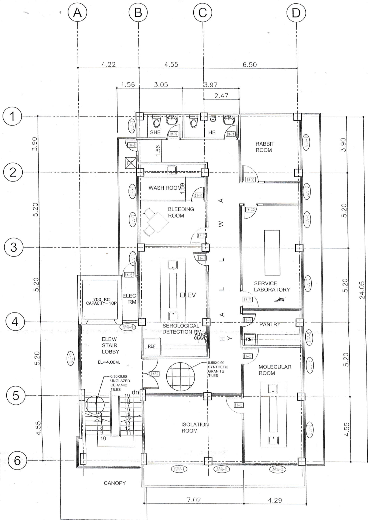
2 SECOND FLOOR PLAN A-2 NOT TO SCALE
