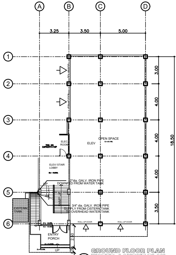
1 GROUND FLOOR PLAN WATER LAYOUT PLAN SCALE 1 : 100 M
