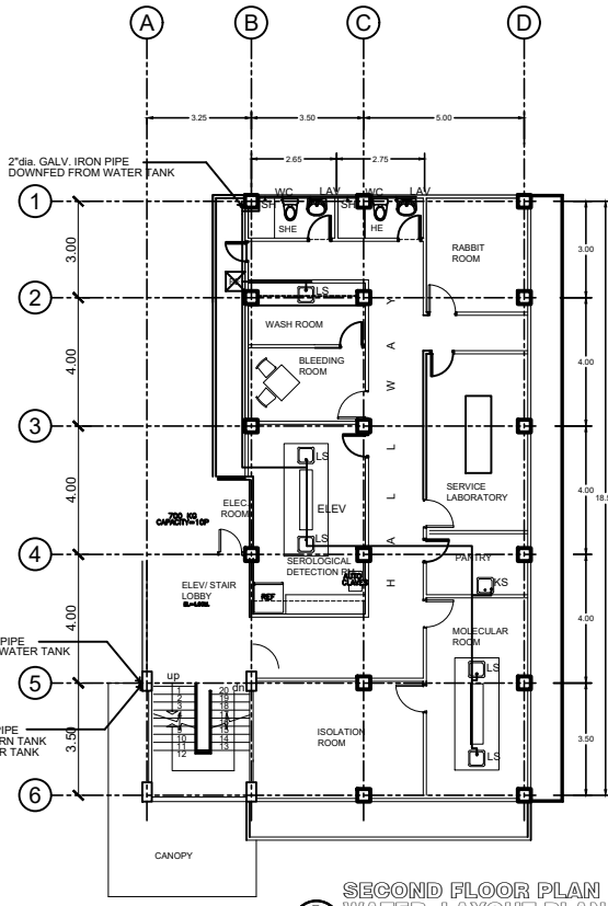
2 SECOND FLOOR PLAN WATER LAYOUT PLAN SCALE 1 : 100 M
