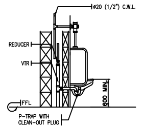
5 DET. AT URINAL SCALE 1 : 50 M
