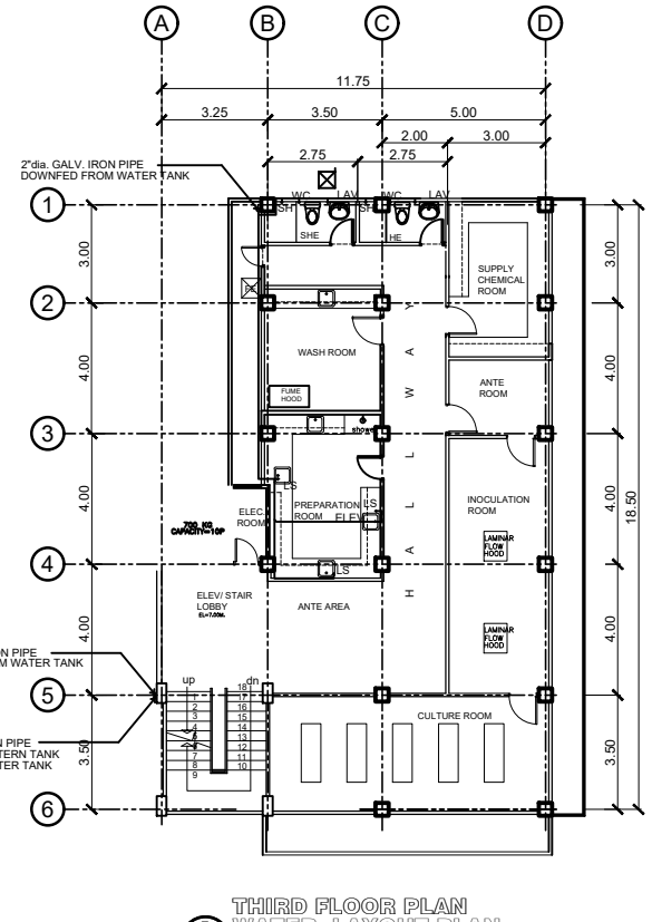
3 THIRD FLOOR PLAN WATER LAYOUT PLAN SCALE 1 : 100 M
