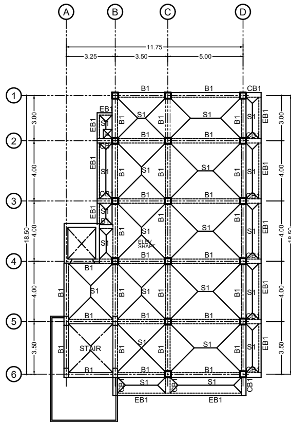
2 S-1 SECOND FLOOR FRAMING PLAN SCALE 1:100 M
