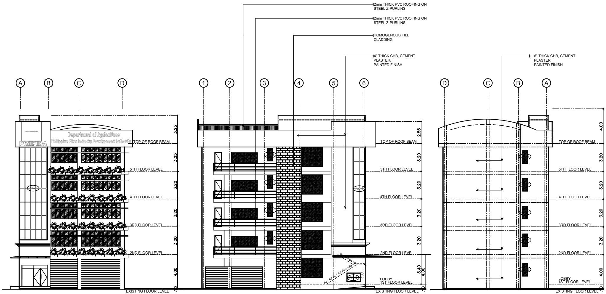
1 FRONT ELEVATION SCALE 1:100 M
