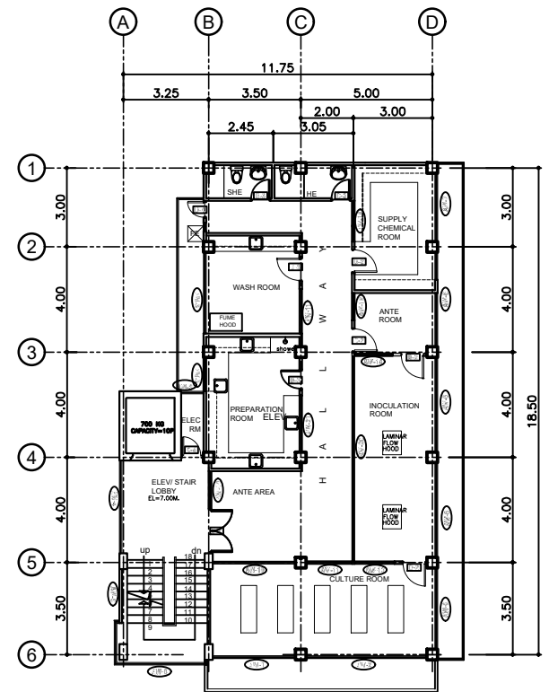
3 THIRD FLOOR PLAN SCALE: 1:100 M
