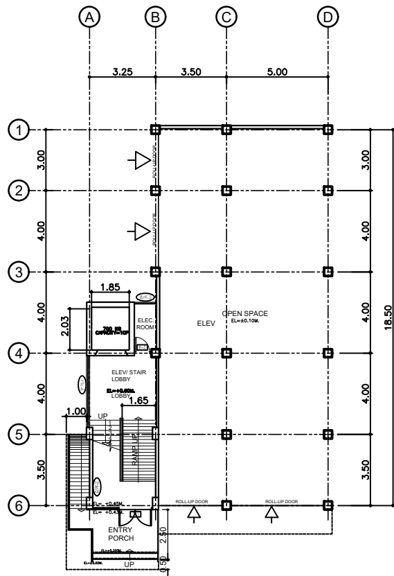
1 GROUND FLOOR PLAN SCALE: 1:100 M
