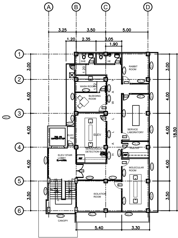
2 SECOND FLOOR PLAN SCALE: 1:100 M
