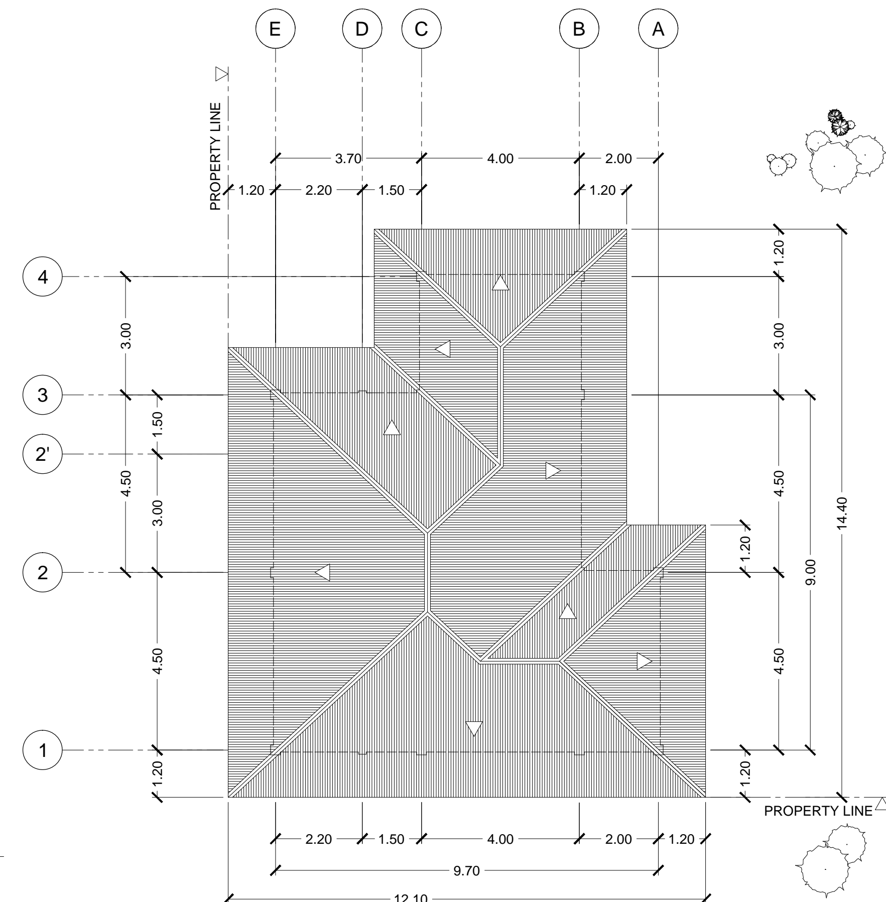
1 SITE DEVELOPMENT PLAN A - 1 SCALE 1:100 M
