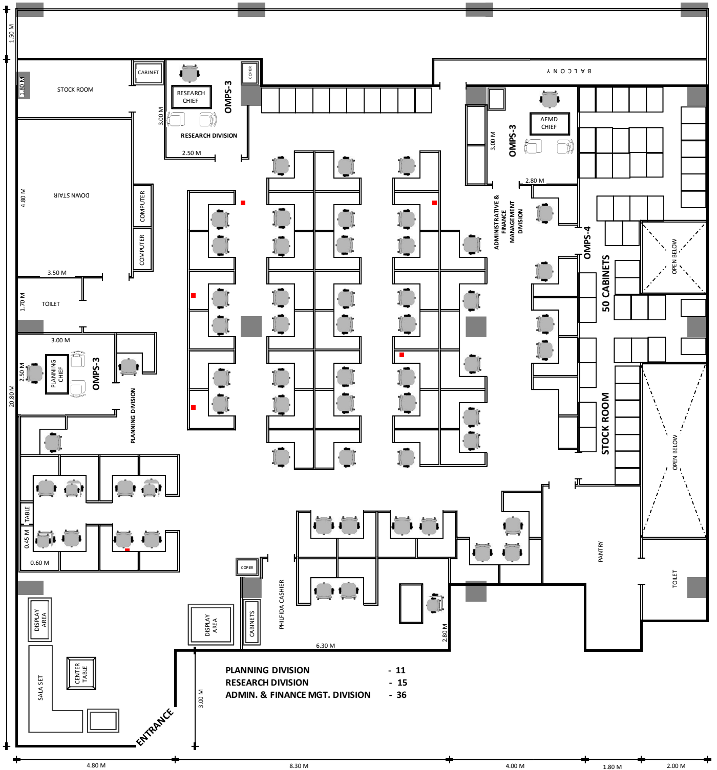
PHILFIDA PROPOSED LAYOUT FOR THE NEW OFFICE BUILDING
