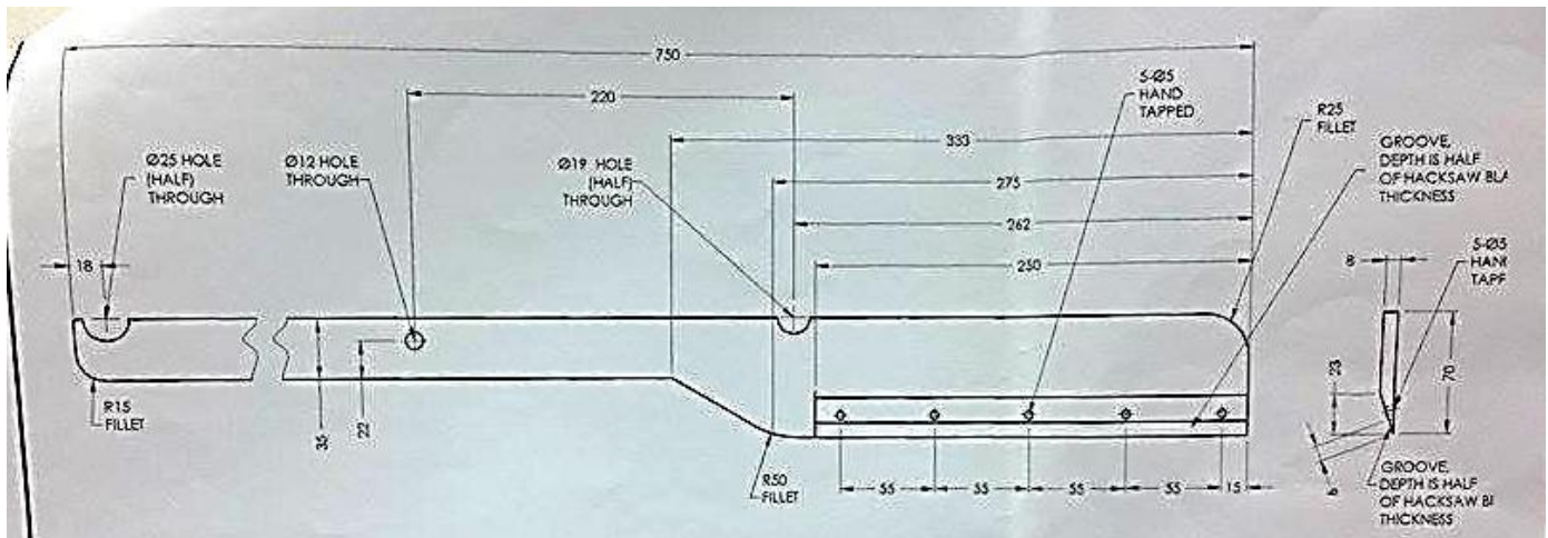
3.1 STRIPPING KNIFE SCALE 1:3 M
